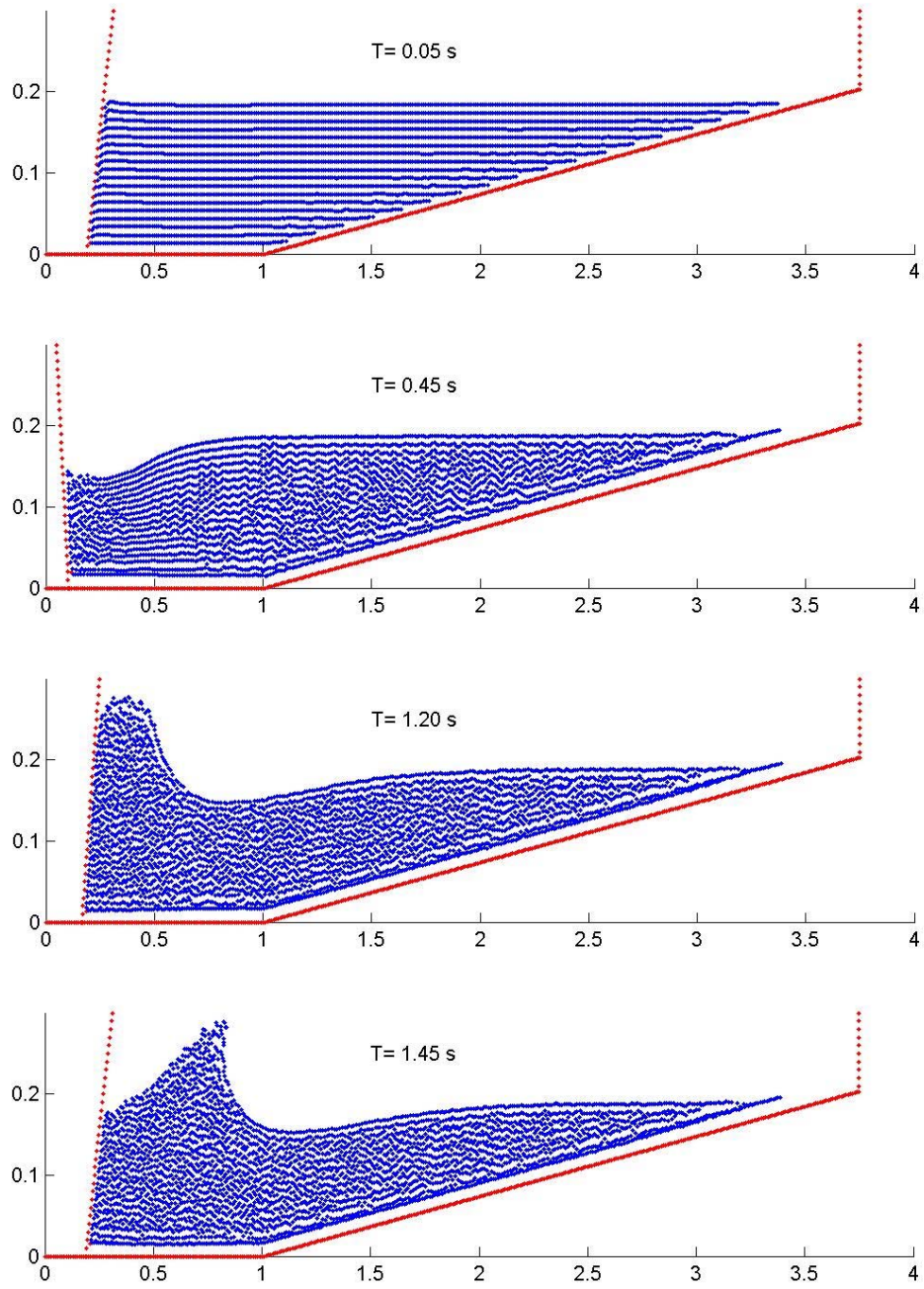
Figure 4.6: Wave formation in Case3 (for 2D).
